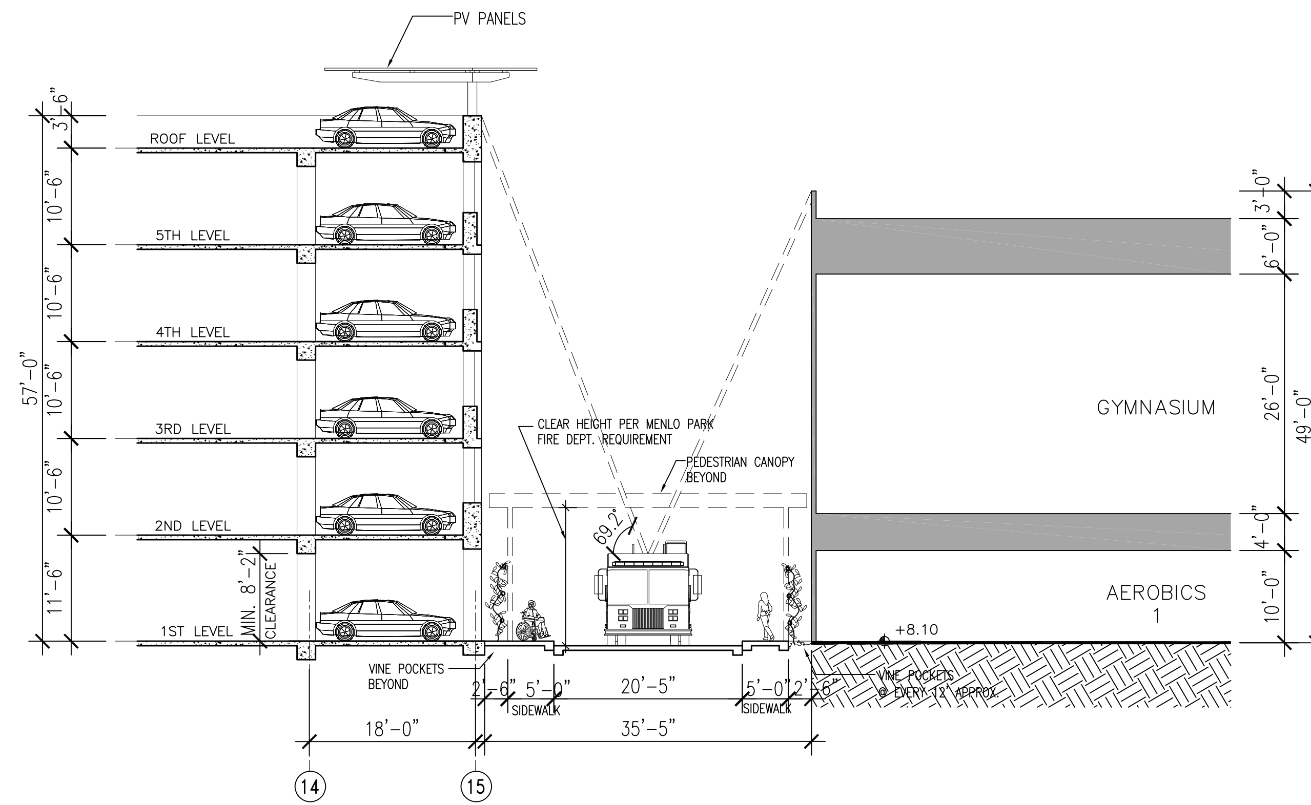
1. SECTION AT FIRE LANE
