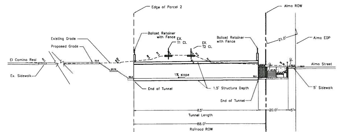
Longitudinal Section through Undercrossing: 1"=16'-0"
